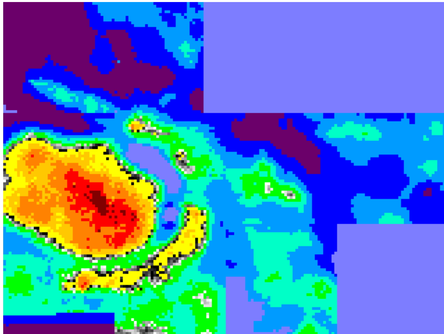
0.5m Twin Probe Earth Resistance Survey Inchnadamph, Sutherland October 2005
