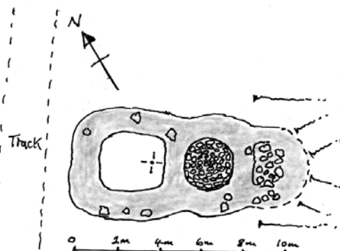
AUCHTERTIPPER - MOOR SITE JW3 CENTRED ON: 292653 828567 CORN/MALT KILN & BARN DATE 11/10/2010 DRAWN AT 1:200 BY JLD
