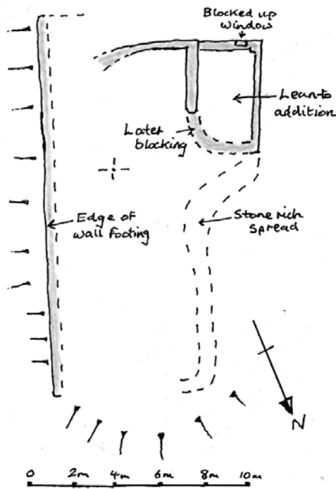
ESS FARMSTEAD SITE LM12 RUINS OF SEVERAL BUILDINGS CENTRED ON: 292 817 827242 DATE 15/10/2010 Drawn by: L.G.J. At 1:200
