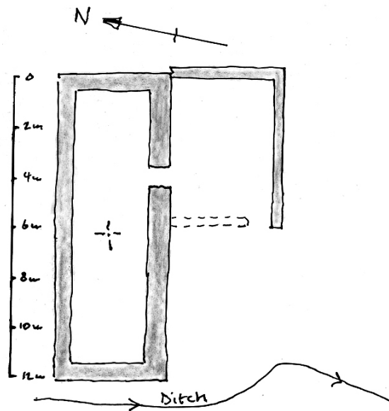
BADENARGIT FARMSTEAD (EAST) SITE: JW15 CENTRED ON: 292183 826260 STONE FOOTINGS OF A BUILDING Date 18/10/2010 Drawn by J.F.O. at 1:200
