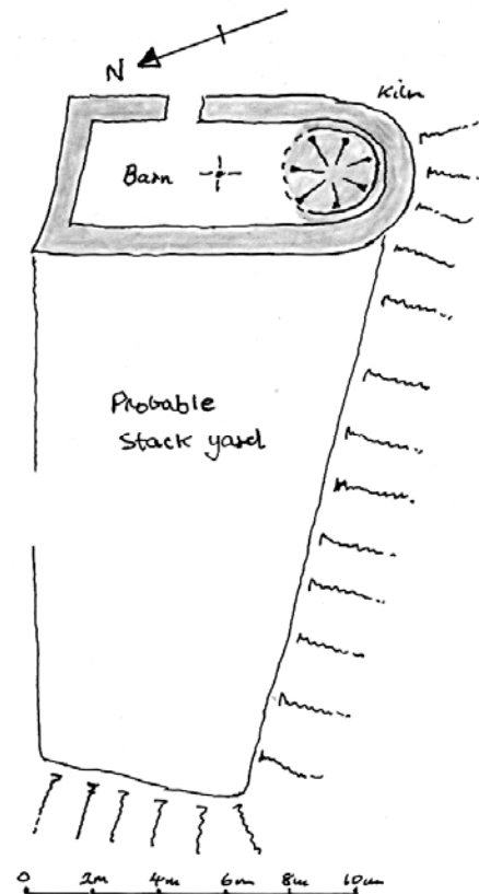
AUCHTERTIPPER FARMSTEAD SITE JW7 CORN KILN, BARN & STACK YARD DATE: 11/10/2010 DRAWN AT: 1:200 BY JLD CENTRED ON: 293004 828935
