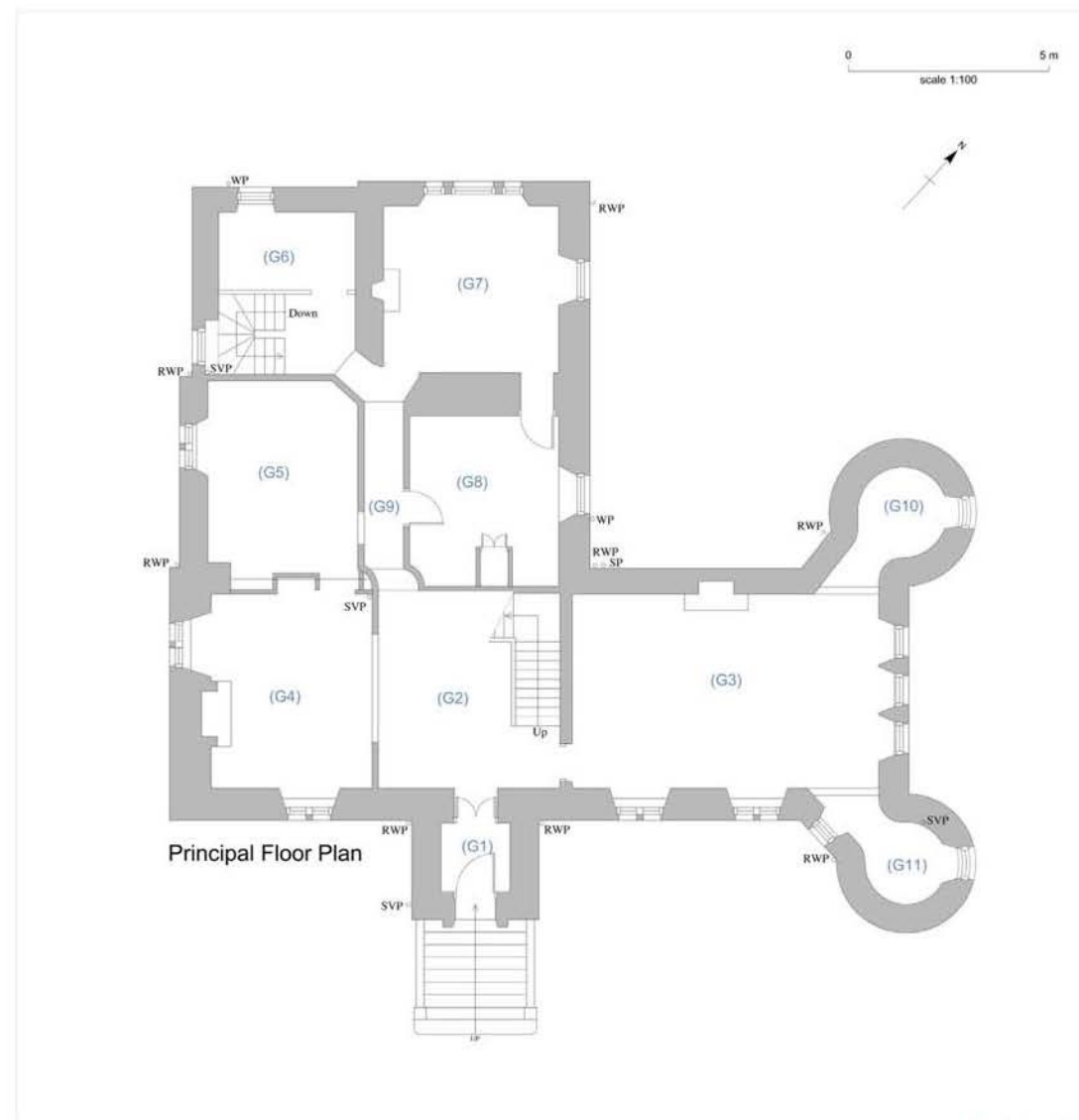
ground floor plan with room numbers
