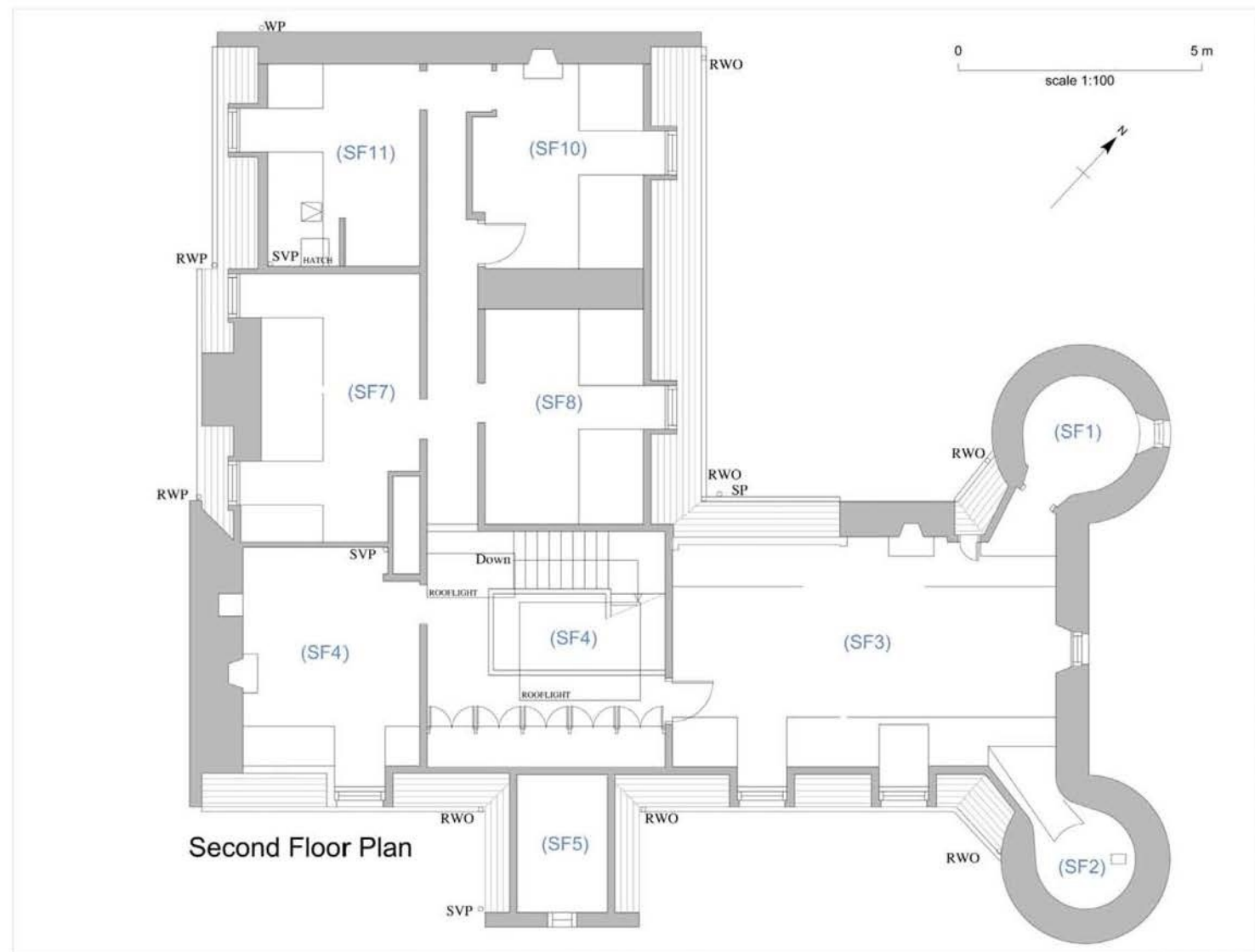
second floor plan with room numbers
