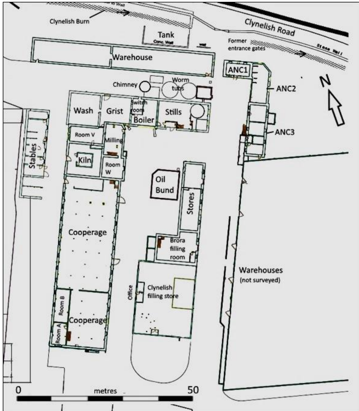
Figure 4 – The Clynelish Old Distillery buildings, structures and rooms. Scale shown
